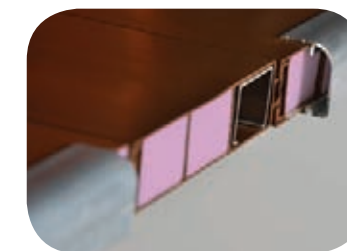
Aluminum Channel & Closed-Cell Owens Corning Foam Interior
